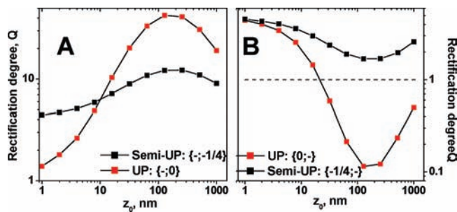
Figure 6. Comparison of unipolar diodes (UP), which consist of a charged zone and a zone that is neutral, to semi-UP diodes, which consist of two zones with a surface charge of the same sign but different density. As evidenced by our experiments, a neutral surface ( \sigma = 0 ) is difficult to achieve for our pores; we calculated current–voltage curves when 75% of the surface carboxyls were converted to uncharged methoxy groups. A) Comparison of the rectification degree for \{-,0 and \{-;1/4- diodes. B) Rectification degrees Q for \{0,- and \{1/4-;- diodes. As followed from this figure, semi-UP conical diodes are very similar in their behavior to initial conical pores, thus devices with the surface charge pattern \{-;- . The calculations were performed for L = 12 \mu\text{m} , A = 250 \text{ nm} , C_{\text{bulk}} = 0.1\text{M} , and \sigma = -0.5 \text{ e/nm}^2 . The rectification degree was calculated for 1 V. See text for details.
