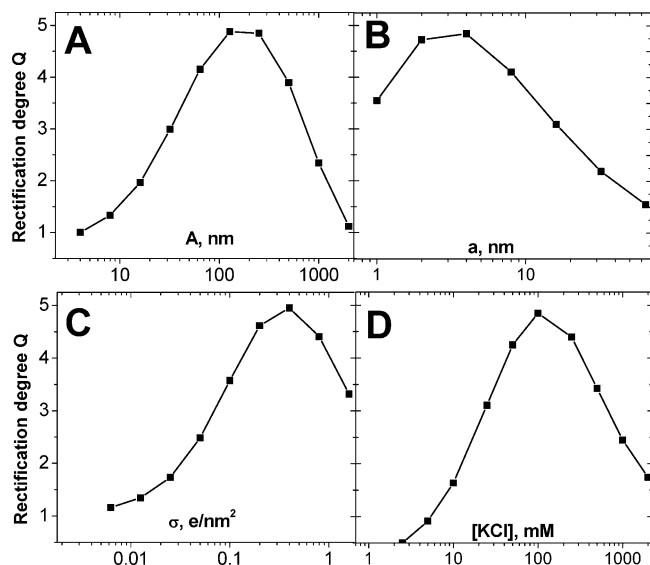
Figure 2. Numerically calculated rectification degrees (eq 1 at 1 V) of a homogeneously charged conical nanopore as a function of A) base radius, A B) tip radius, a C) surface charge, \sigma , and D) bulk concentration of KCl. The following values were used C_{\text{bulk}} = 0.1 M, \sigma = -0.5 e/nm 2 , A = 250 nm, a = 4 nm, and L = 12 \mu\text{m} , unless the parameter was varied. The calculations were performed by numerically solving the 3D Poisson–Nernst–Planck equations. Our analysis showed that it was impossible to achieve rectification degrees higher than 5 for the examined range of the varying parameters, at least for our experimental nanochannel length of L = 12 \mu\text{m} . Note that every graph has a maximum due to the interplay of the Debye length and the polarization effect at the nanopore entrance (including access/Hall resistance).
