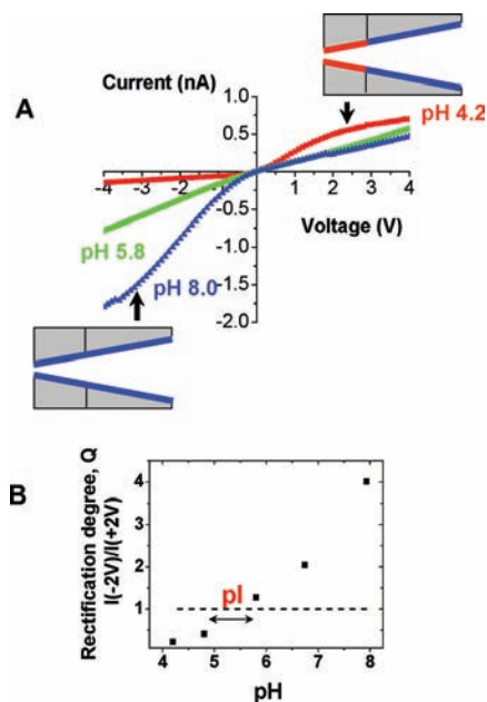
Figure 8. Functioning of a diode sensor for streptavidin. A) Experimental current–voltage curves for a single conical nanopore whose tip was modified with biotin and exposed to 0.5 \mu\text{M} solution of streptavidin. The measurements were performed in 10 mM KCl and various pH conditions, at which streptavidin was positively charged (pH 4.2, red squares), negatively charged (pH 8.0, blue triangles), or neutral (pH 5.8, green squares). B) Rectification degree measured at different pH for a single conically shaped nanopore with biotin and streptavidin at the tip. The current–voltage curve flipped at the value of pH that corresponds to the protein isoelectric point (pI). Dashed line (---) is a guide to the eye showing Q = 1 , i.e. no rectification. The value of pI for surface-immobilized streptavidin as determined by our biosensor is \sim 5.5 .
