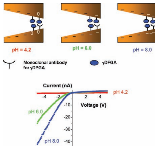
Figure 10. Sensing \gamma DPGA with a nanopore that contained mAb F26G3 at the tip. A nanopore with mAb F26G3 was incubated with a solution of \gamma DPGA for 3 h, and the current–voltage curves were measured in 10 mM KCl. Depending on pH of the solution, different surface charge patterns were formed on the pore walls (the schematics in the upper part of the figure), which led to different current–voltage curves. At pH > 4, the polypeptide was negatively charged and thus the current–voltage curves reversed compared to the situation before the \gamma DPGA binding (Figure 9).
