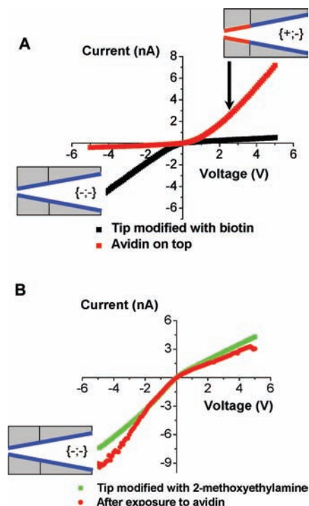
Figure 7. Functioning of a nanofluidic diode sensor for avidin. A) Experimental current–voltage curves for a conical nanopore whose tip was modified with biotin before exposure to avidin (■), and after exposure to 0.5 \text{ }\mu\text{M} solution of avidin (red ■). The current–voltage curves were measured in 10 \text{ mM KCl} solution, \text{pH} = 5.5 . The insets indicate the schematics of obtained surface charge patterns. Binding of avidin to the biotin modified pore resulted in the formation of the bipolar diode surface charge pattern. B) Studies of nonspecific adsorption of avidin to a nanopore whose tip was modified with 2-methoxyethylamine. The current–voltage curve of this pore did not significantly change upon exposure to avidin, suggesting that nonspecific interactions of the protein with the pore walls do not influence functioning of the sensor.
