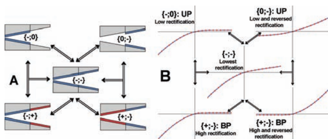
Figure 3. Schemes of various surface charge patterns that could lead to preparation of ionic diodes together with their current–voltage curves. The arrows indicate possible transitions between different surface charge patterns, which can be induced upon binding of one type of analyte to the pore walls. A) Schematics of unipolar (UP) diodes are in the upper row, whereas bipolar diodes (BP) are shown in the bottom row. A homogeneously charged conical nanopore is shown in the middle. B) Behavior of current–voltage curves of the nanopores shown in (A). BP diodes have superior rectification properties compared to UP diodes, that is BP diodes produce higher rectification degrees. A conical nanochannel with homogeneous surface charges shows the lowest rectification degree. Note that, in the transition from a homogeneously charged conical nanopore to the {+;-} and {0;-} configurations, the current–voltage curve flips, which allows for a very easy detection of the analyte that induced this change. See text for details.
