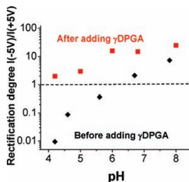
Figure 11. Sensing bacterial polyglutamic acid ( \gamma DPGA) with a nanofluidic diode – summary of Figures 9 and 10. Rectification degree for 5 V is shown as a function of pH. Dashed line (---) is a guide to the eye showing no rectification, i.e. Q = 1 . Rectification direction at acidic pH for a nanopore modified with mAb F26G3 (■) is reversed compared to the rectification of the same pore after exposure to \gamma DPGA (red ■). See text for details.
