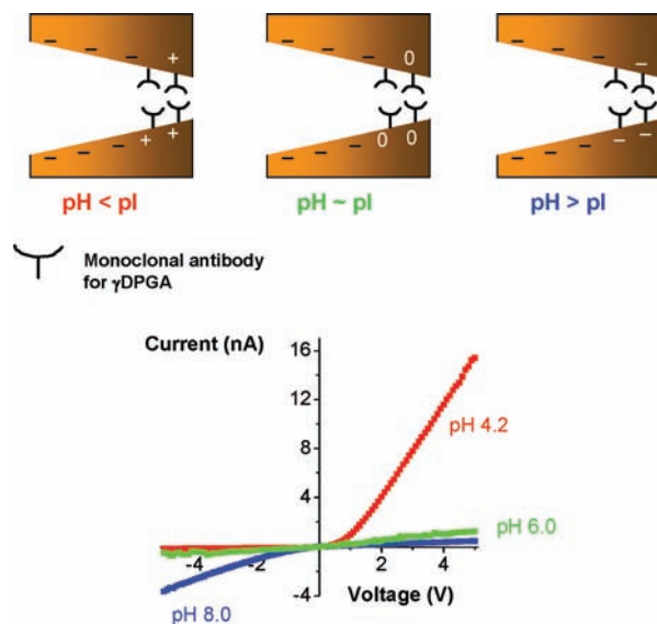
Figure 9. Determination of the isoelectric point of the monoclonal antibody for the bacterial polyglutamic acid ( \gamma DPGA). Current–voltage curves were recorded for a conical nanopore whose tip had been modified with a monoclonal antibody (F26G3) to the bacterial \gamma DPGA. The measurements were performed in 10 mM KCl and at various pH values. At acidic pH conditions, the antibody F26G3 was positively charged (red recordings), whereas at basic pH it was negatively charged (blue recordings). The system stopped rectifying at pH \sim 6.0 (green recordings), which corresponded to pI of the antibody. The schemes show various surface charge patterns that were created at the three studied pH values. The uneven surface charge pattern was created at acidic pH values, which caused the formation of a strongly rectifying bipolar diode.
