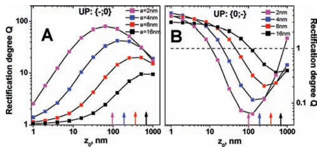
Figure 5. Numerically calculated rectification degrees of conical unipolar (UP) diodes as a function of the transition zone location ( z_0 ) and the tip radius ( a ). The arrows show the position of the transition zone that assures the highest rectification degree, as estimated by eq 4. Rectification degrees of the device whose tip is charged and the base is uncharged – \{-;0\} . B) Rectification degrees for the \{0;- device. The calculations were performed for L = 12 \mu\text{m} , A = 250 \text{ nm} , C_{\text{bulk}} = 0.1\text{M} , and \sigma = -0.5 \text{ e/nm}^2 .
