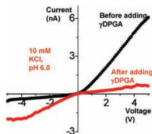
Figure 12. Studies of nonspecific adsorption of \gamma DPGA to nanopores with positively charged tip. A single nanopore was asymmetrically modified at the tip with avidin and exposed to a solution containing \gamma DPGA. Nonspecific adsorption caused a flip of the current–voltage curve; however, the recorded negative currents were significantly lower than the currents observed upon binding of \gamma DPGA to a nanopore that contained mAb F26G3 (Figure 10). The measurements were performed in 10 mM KCl, pH 6.0.
